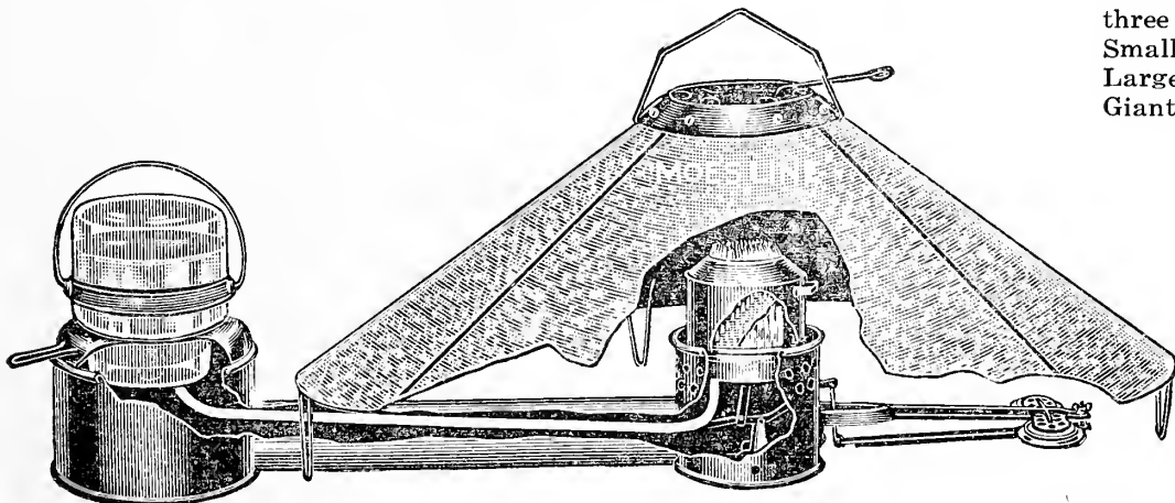
Moe's No. 226 Automatic Oil Burning Hover
